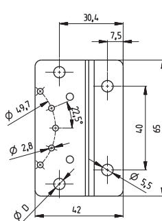
Bracket type B
